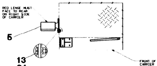
VIEW H-H
